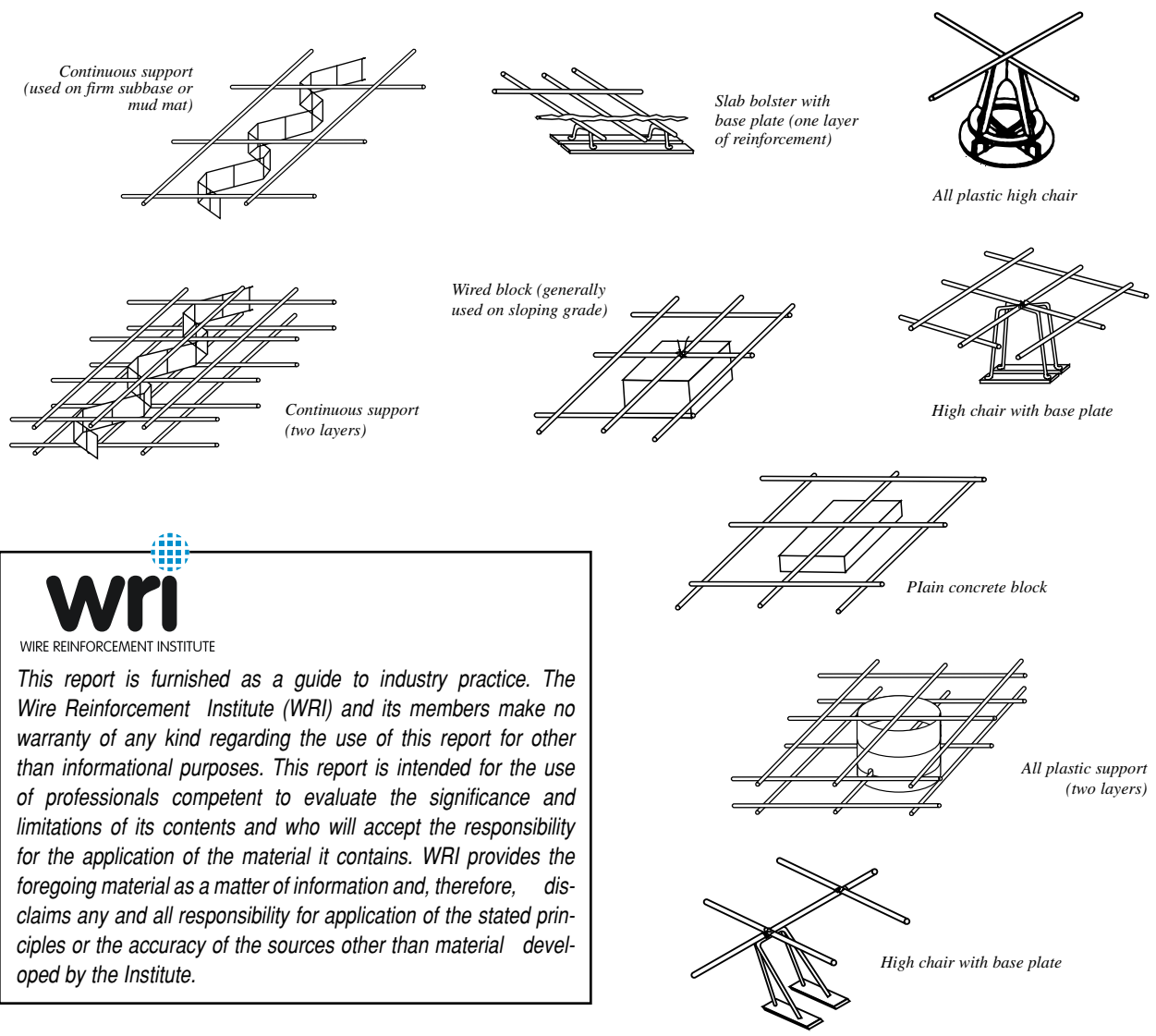
FIGURE 1 — TYPES OF SUPPORTS
